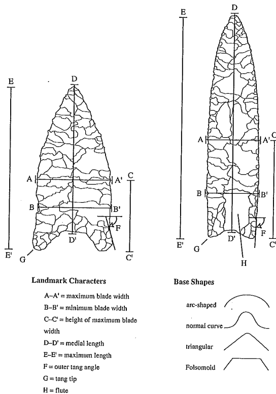
Figure 4.9. Phylogenetic ordering of prehistoric projectile points from the southeastern United States (after O'Brien et al. 2002). The ordering in (a) was created using the eight landmark characters shown in (b); character states not shown. Only a portion of the phylogenetic tree is shown here. The complete tree has a length of 22 and a consistency index of .59 (after O'Brien et al. 2001; O'Brien et al. 2002).
