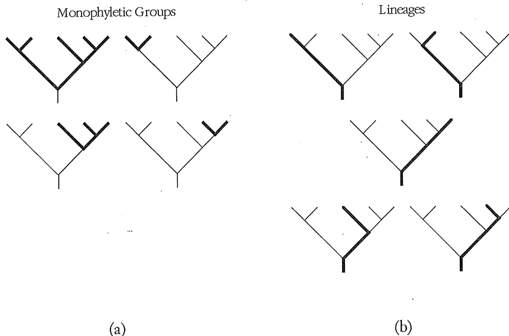
Figure 4.10. Diagrams showing the difference between monophyletic groups and lineages (after de Queiroz 1998). All nine diagrams represent the same phylogeny, with monophyletic groups highlighted on the left and lineages on the right. Additional lineages can be counted from various internal nodes (ancestors) to the branch tips (descendants).
