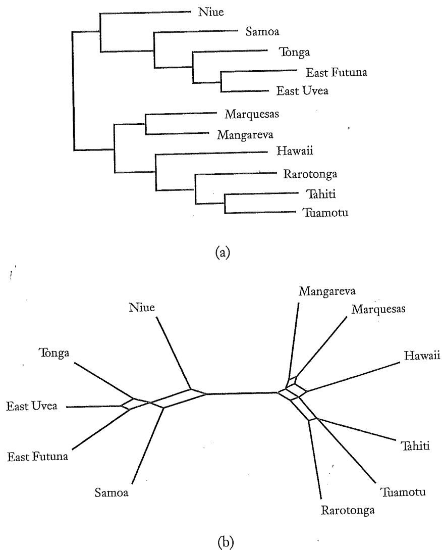
Figure 4.5. Detecting potential borrowing among 11 Polynesian languages (after Hurles et al. 2003). In (a) the languages are arranged on a parsimony tree; in (b) they are arranged in a splits graph to show borrowing that took place within the western (blue) and eastern (red) Polynesian clades.
